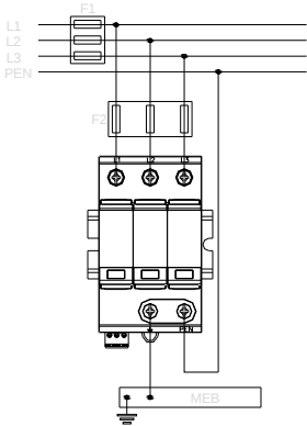
Three-phase TN-C system
